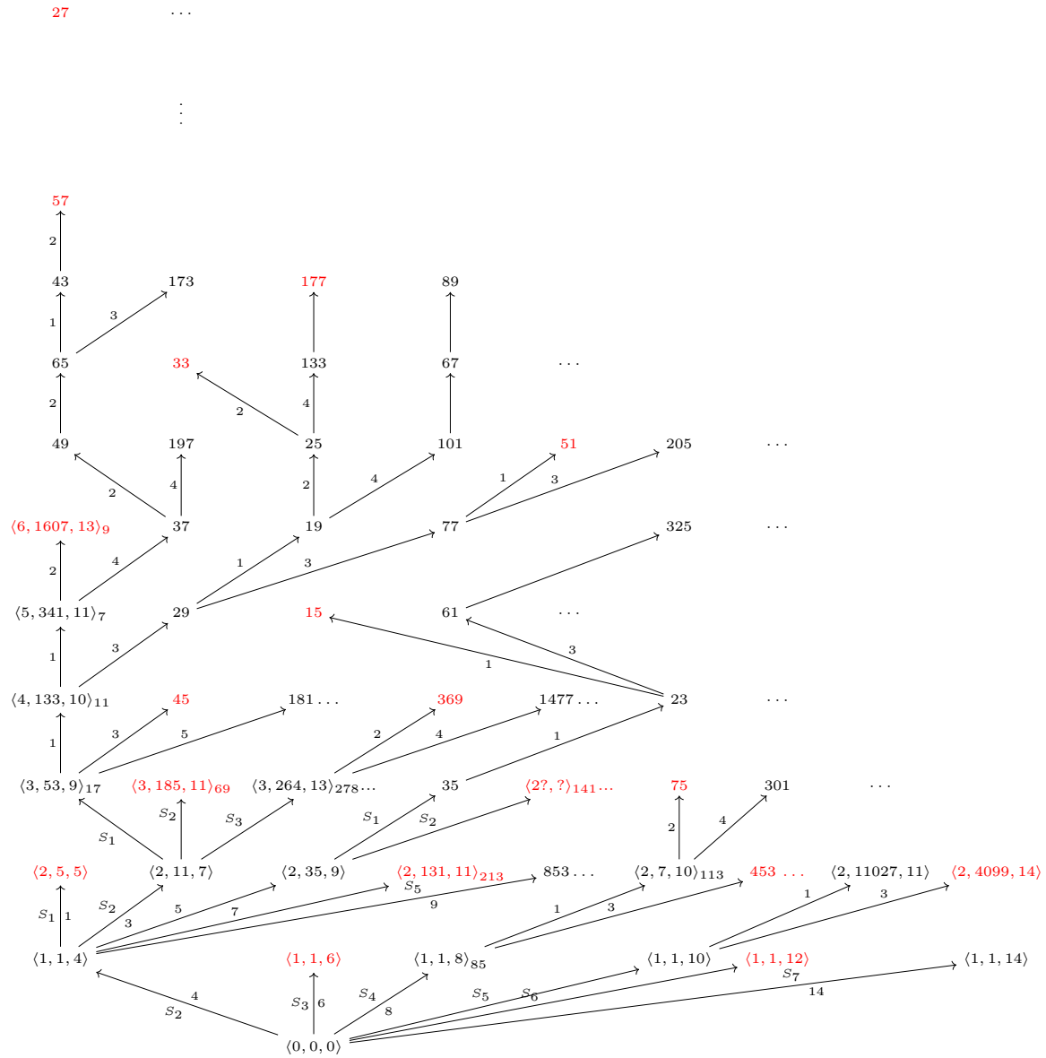
Figure 12. A fragment of the tree \mathcal{F}
