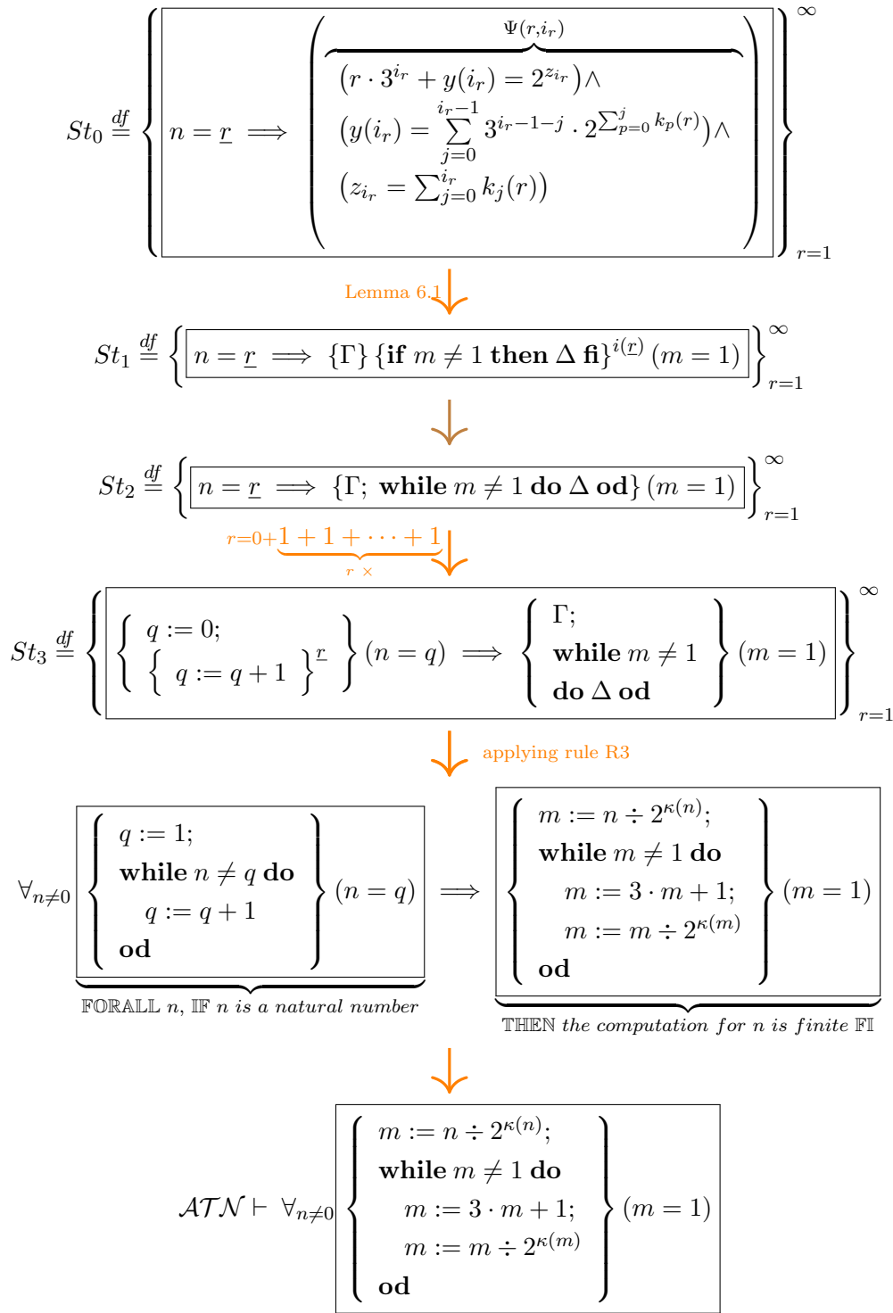
Figure 11. Structure of the proof
