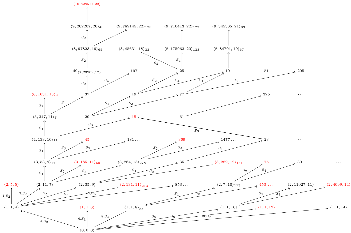
Figure 13. Fragment drzewa \mathcal{F}
